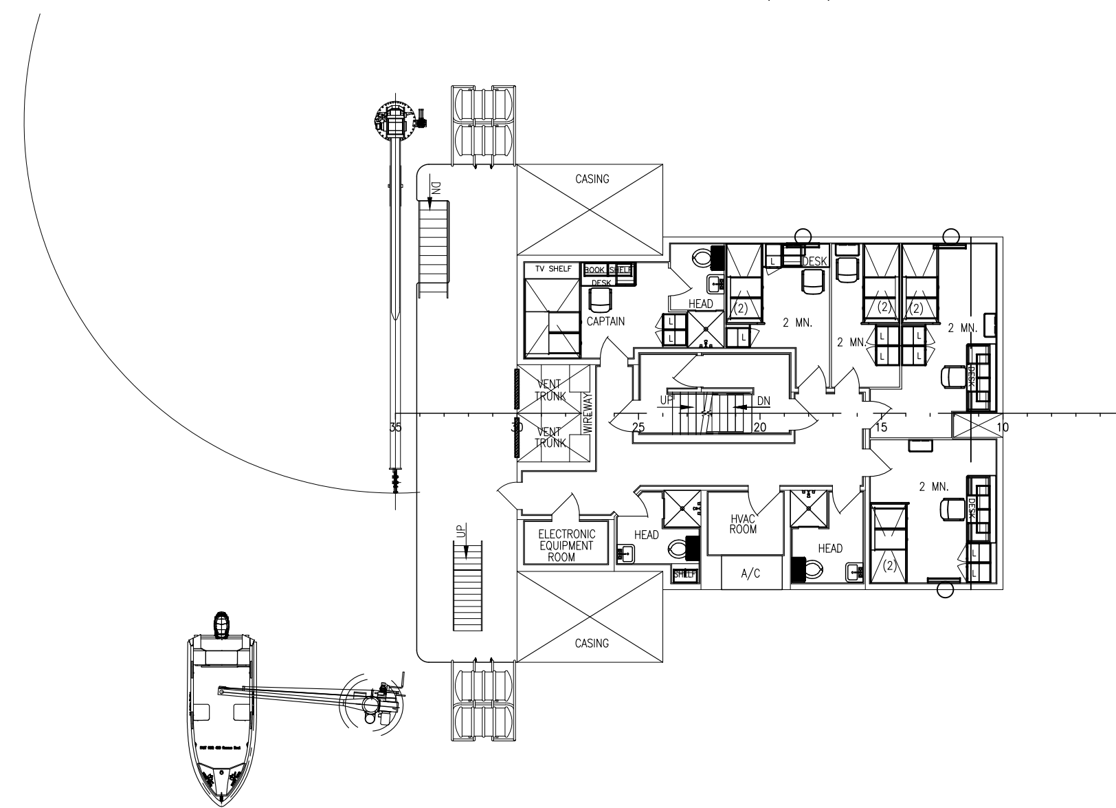
02 DECK PLAN 42'-5 5/8" ABL
