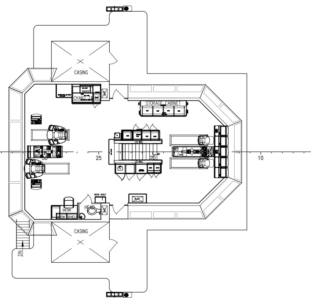
03 DECK PLAN BRIDGE - 51'-4 5/8" ABL
