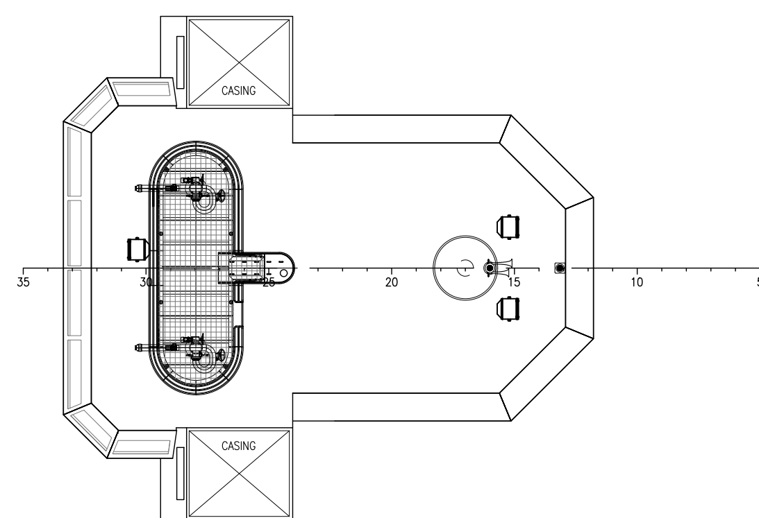
04 DECK PLAN TOP OF HOUSE - 60'-5 1/2" ABL
