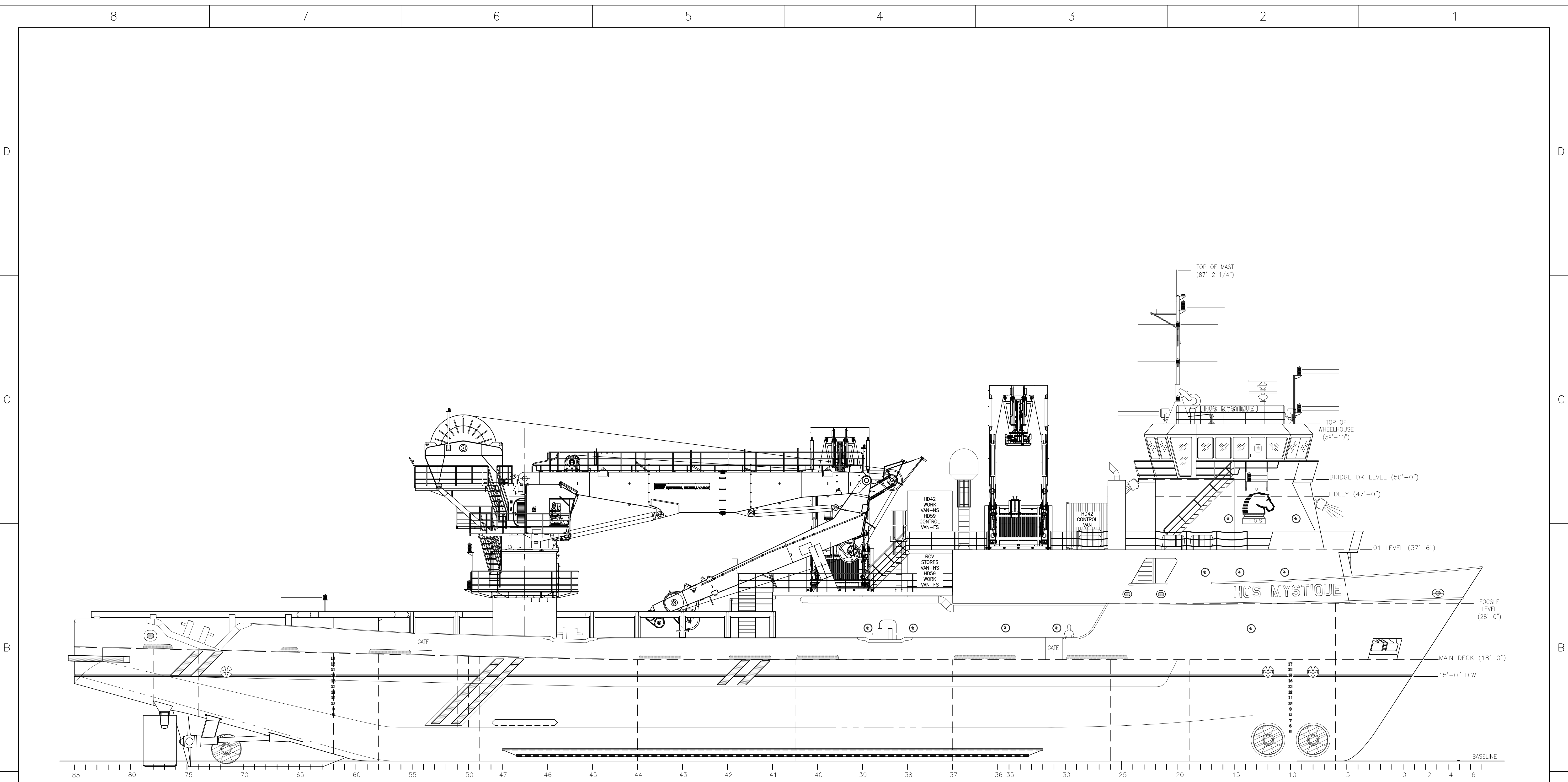
STBD SIDE PROFILE SCALE: 1/8" = 1'-0"
