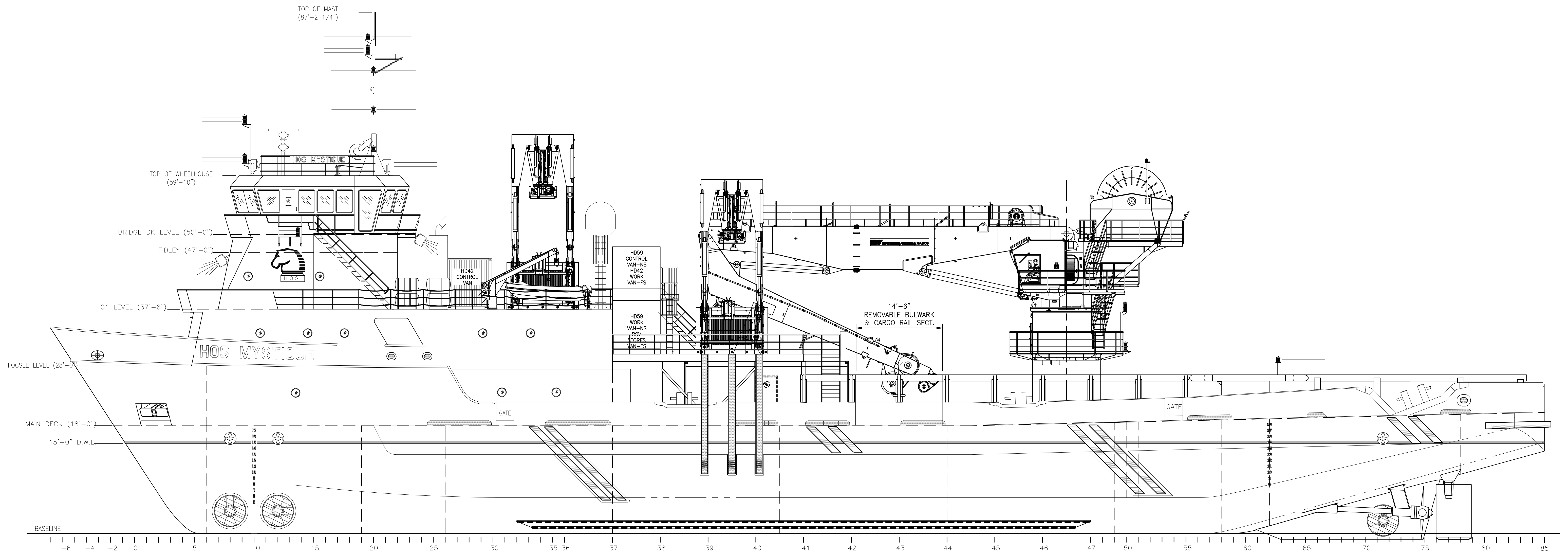
PORT SIDE PROFILE SCALE: 1/8" = 1'-0"
