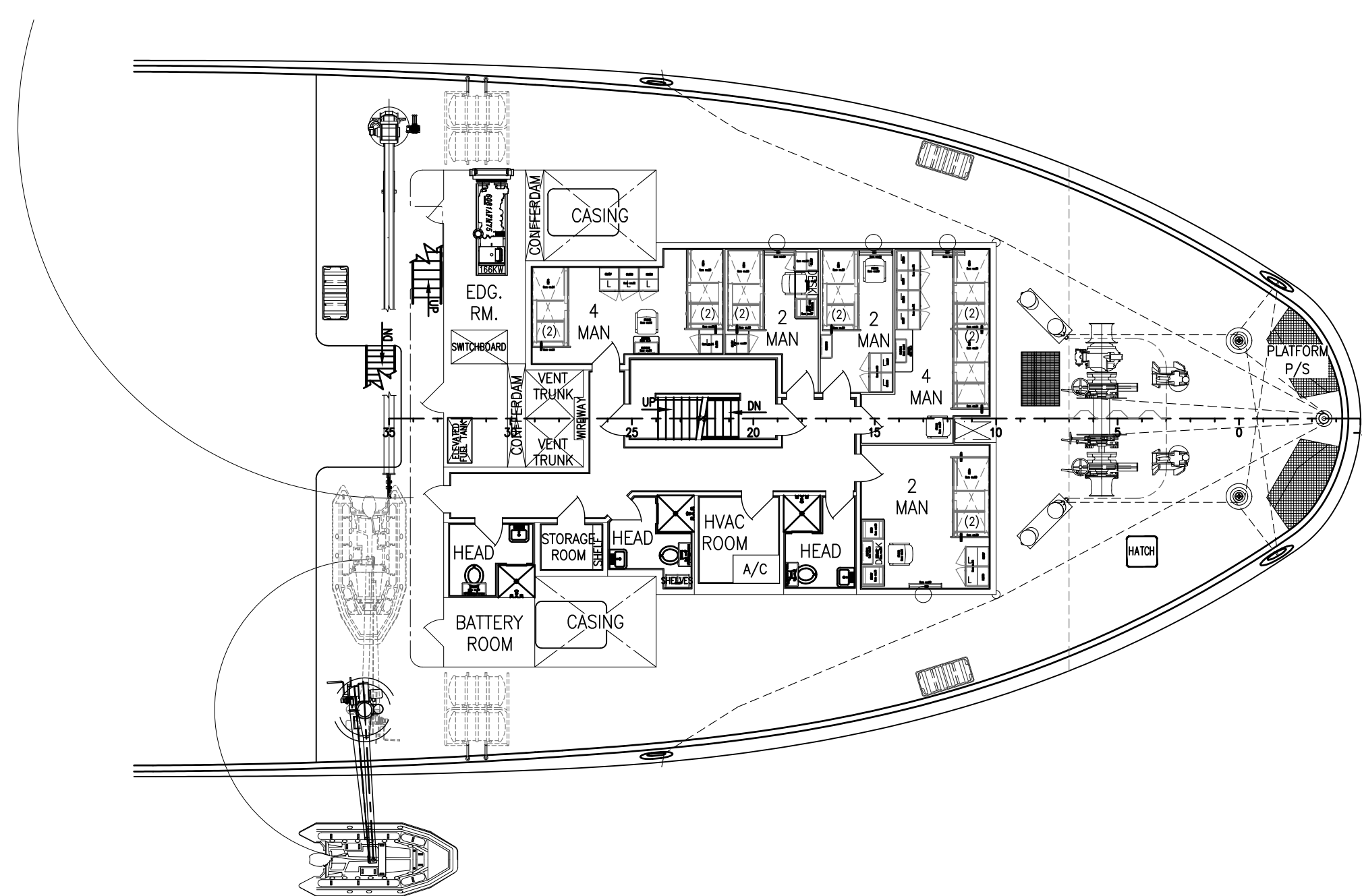
01 DECK PLAN 31'-2" ABL
