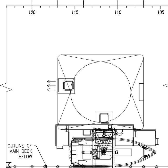
RESCUE BOAT PLATFORM 34'-0" ABL
