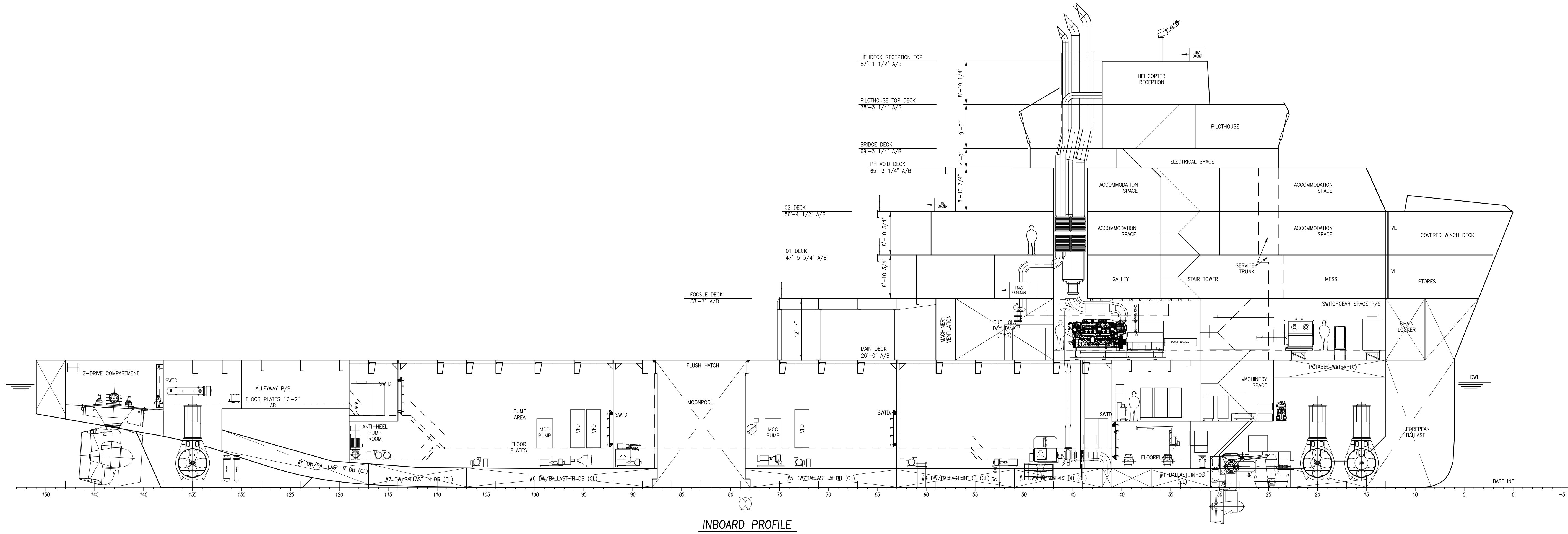
INBOARD PROFILE
