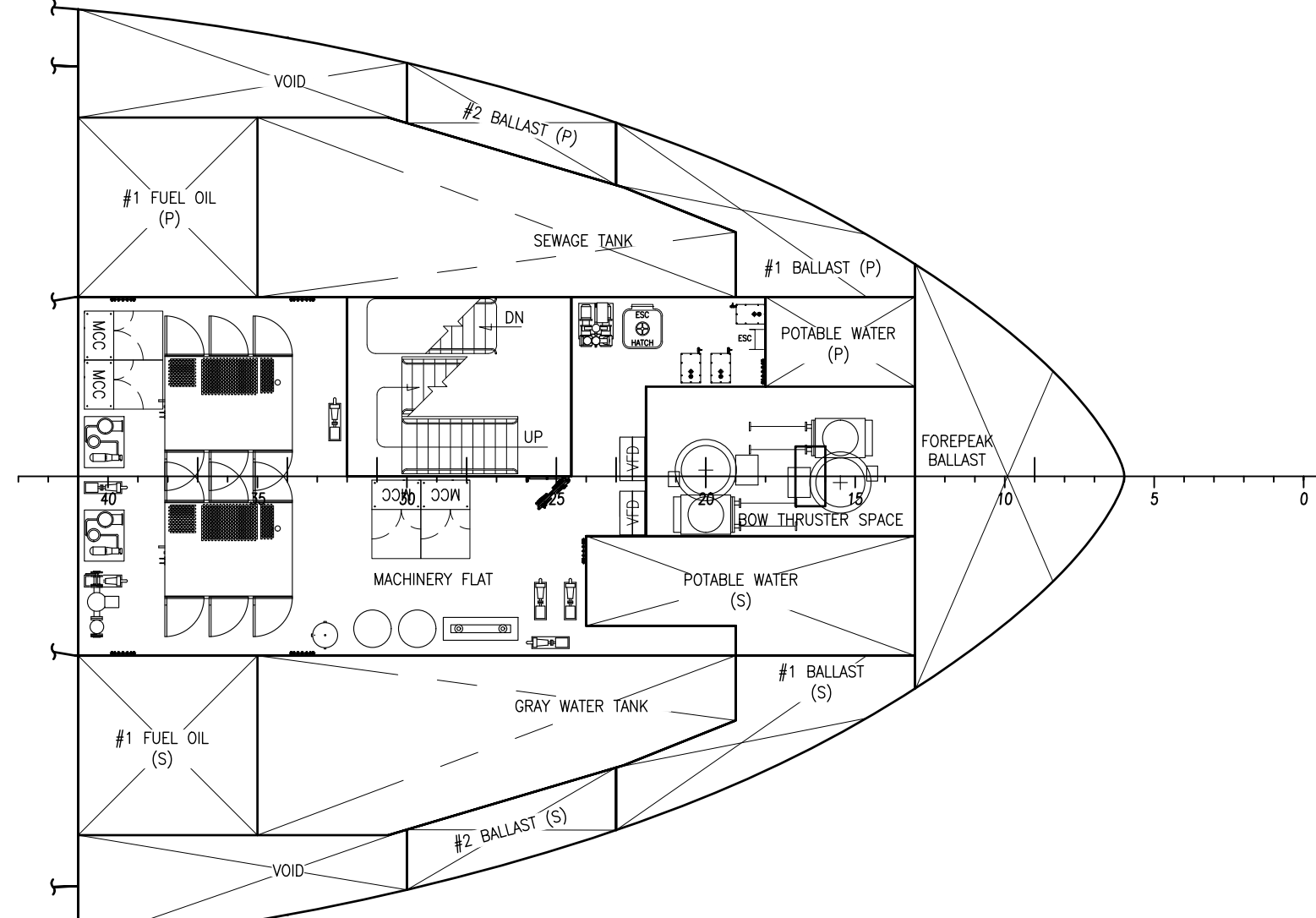
MEZZANINE FLAT
