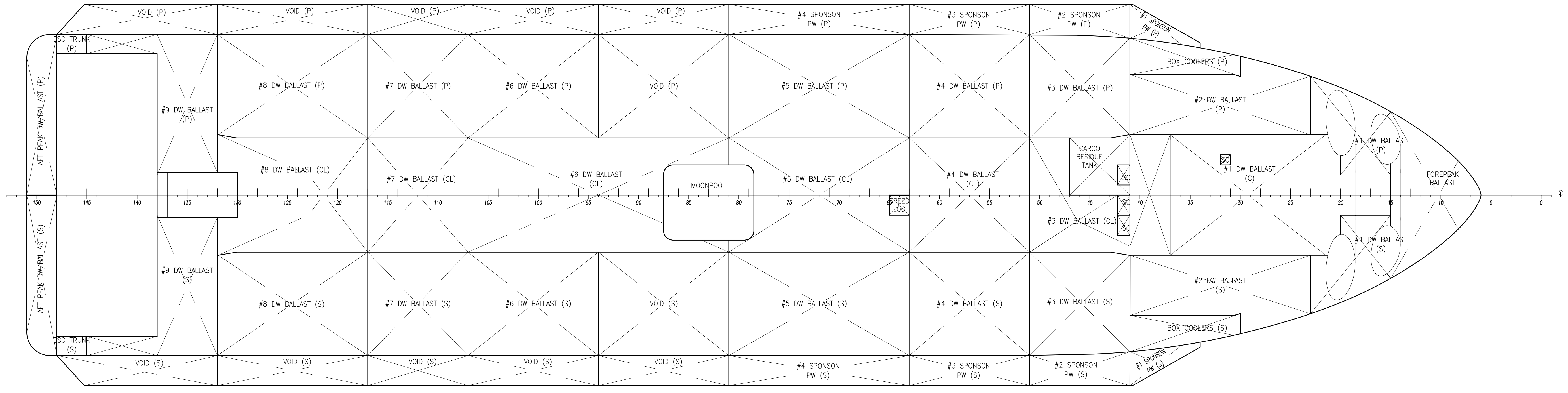
TANK TOP
